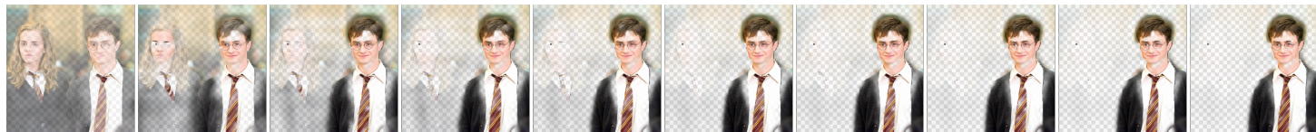
Segmented image
