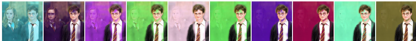
Composite image
