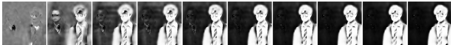
Learnable mask
